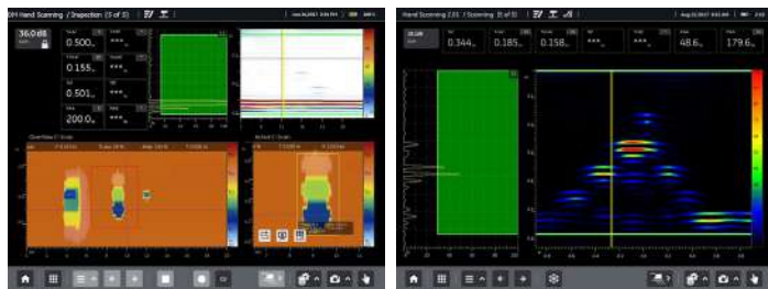
A and E scans, selectable measurements, and touch screen operation
